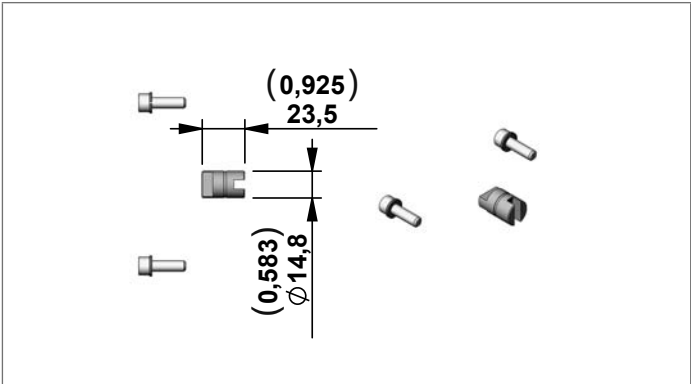
Junction Elements for manifolds ME - MR series
